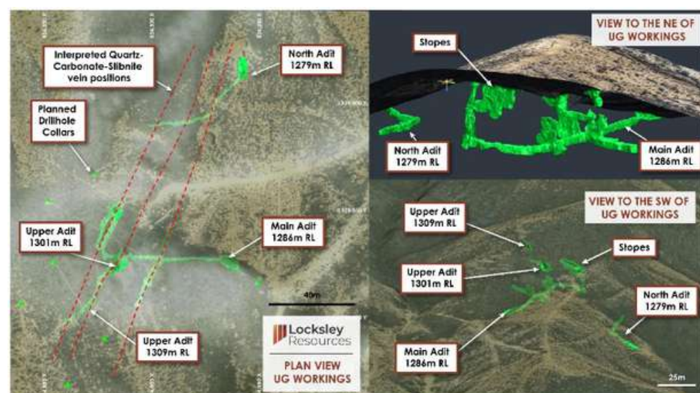
Figure 6: Underground LiDAR survey of the Desert Antimony Mine Workings and interpreted approximate surface position of the Quartz-Carbonate-Stibnite veins.
