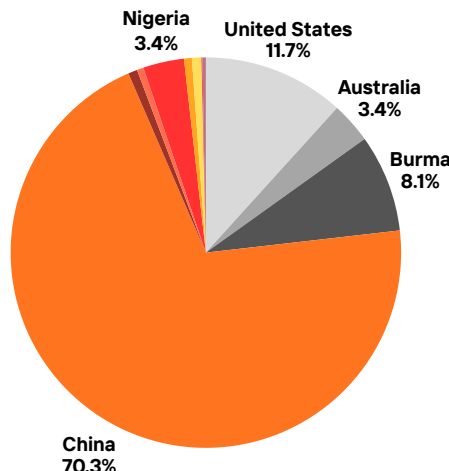
Figure 28: 2024 World rare earth mine production Source: U.S. Geological Survey (2025) Rare Earths
