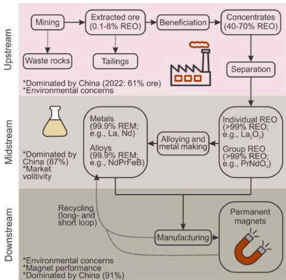
Figure 30: Global supply chain for REOs to produce permanent magnets, Source: Ghorbani et al., (2025) * Denotes current challenges associated with each of the major supply chain streams. Values for Chinese dominance are sourced from USGS (2023) and Wood Mackenzie (2022).
