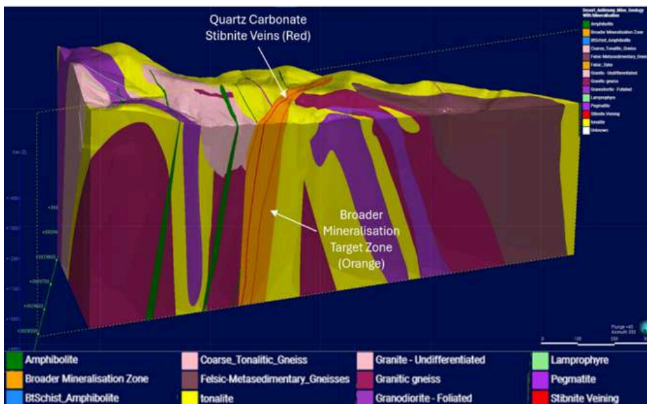
Figure 5: Isometric view to the NE of the 3D geological model which has been constructed from surface geology mapping at the Desert Antimony Mine Prospect. The 'Broader Mineralisation Zone' target horizon is annotated and defined from surface mapping of the occurrence of Stibnite rich Quartz Carbonate Veins. Discrete Stibnite veins have also been modelled and interpreted from surface exposures, Source: Company
